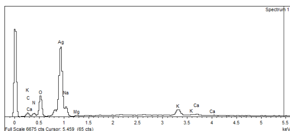
Figure 4: Energy dispersive spectra of the synthesized AgNPs
