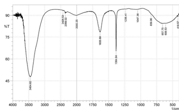
Figure 3: The FTIR spectra of the silver nanoparticles synthesized from Coconut husk extract
