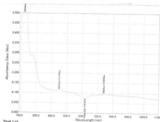
Figure 2: UV-Vis spectra of silver nanoparticles synthesized from Coconut husk extract
